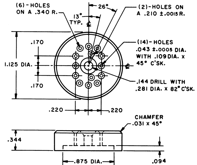
PIN STRAIGHTENER
